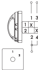
CAM 42 - Voltmetric three concatenated voltages-one of phase
