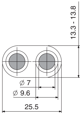
Cable section 25 mm 2 for 63A plugs
