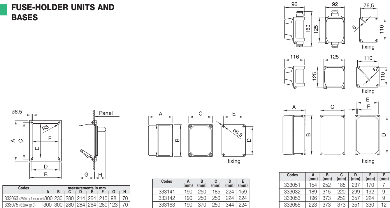
SAFE series - Fuse-holder unit for distribution boards
