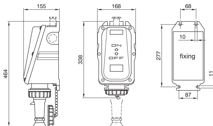
NAVE series - Wall-mounted socket-outlets for containers UNAV 2169
