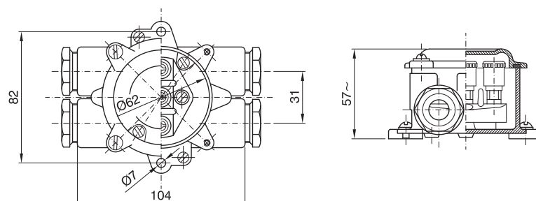
NAVE series - Junction boxes UNAV 1399, UNAV 2161
