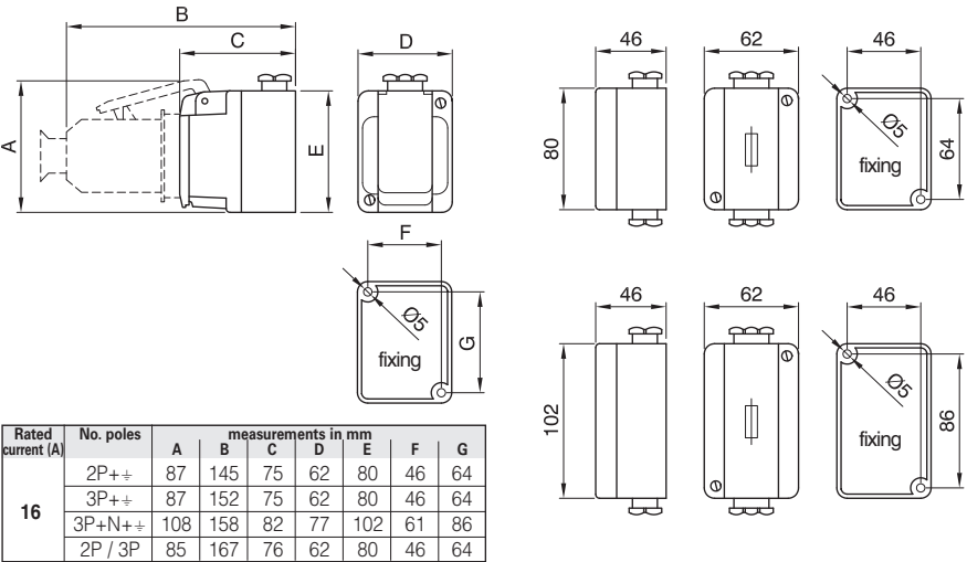
TAIS-MIGNON series Wall-mounting protected industrial socket-outlets
