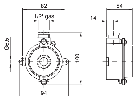
RONDÒ / RONDÒ-Ex series - Push-buttons in wall-mounted watertight enclosures
