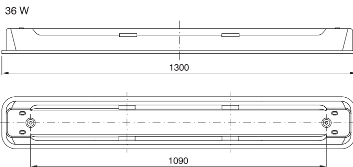
TUNNEL series - Enclosures for tunnel IP66
