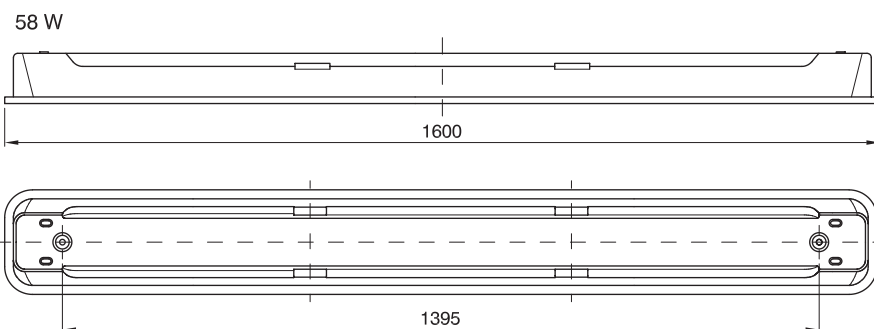
TUNNEL series - Floodlights for tunnel
