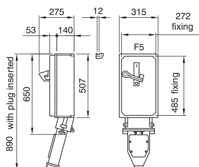
TAIS / TAIS-Ex series - Watertight thermosetting (GRP) control units
