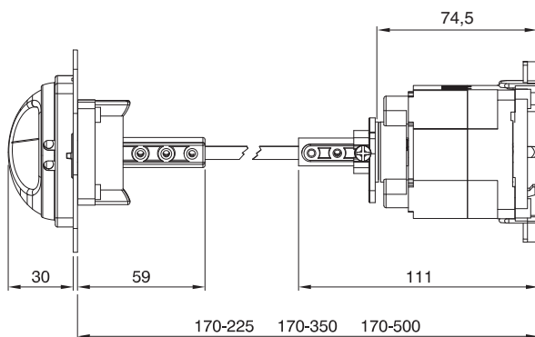
CAM-SZ series - Isolators 16A÷32A with base panel doorlock
