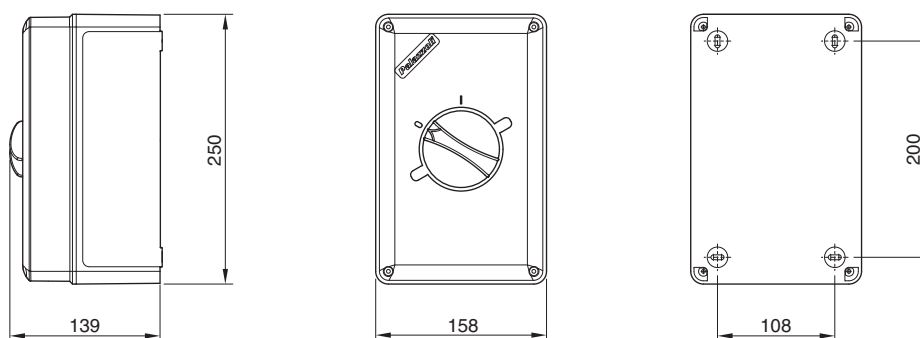
CAM-ST series - 40A and 100A isolator switches in thermoplastic enclosure
