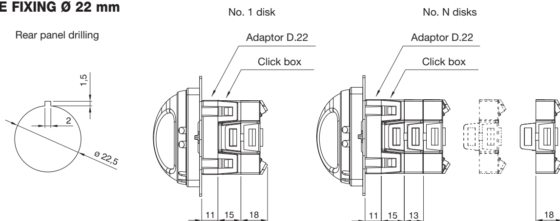
CAM-ST series - Fastening on hole rotary control devices 12/25A
