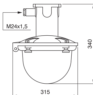
NAUTILUX series - Brass lighting fixtures- IP66
