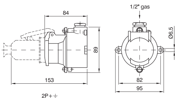
RONDÒ series - Protected wall-mounted industrial socket-outlets
