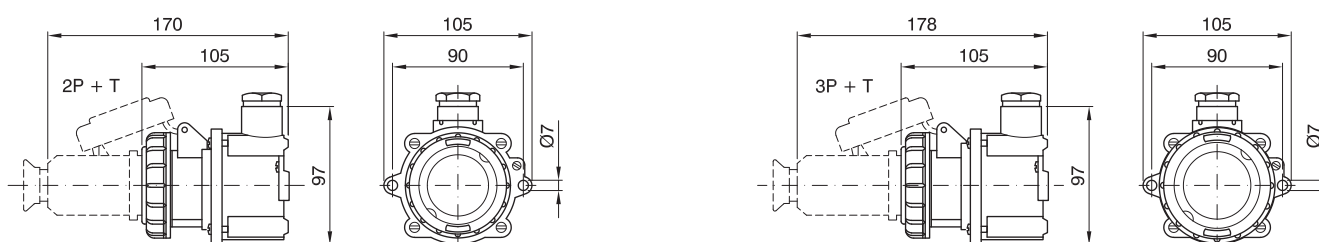
NAVE series - Wall mounted industrial socket-outlets UNAV 2166
