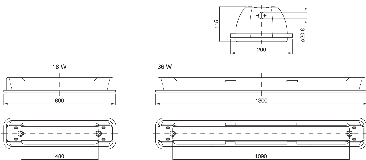
RINO series - Watertight lighting fixtures with polycarbonate diffuser
