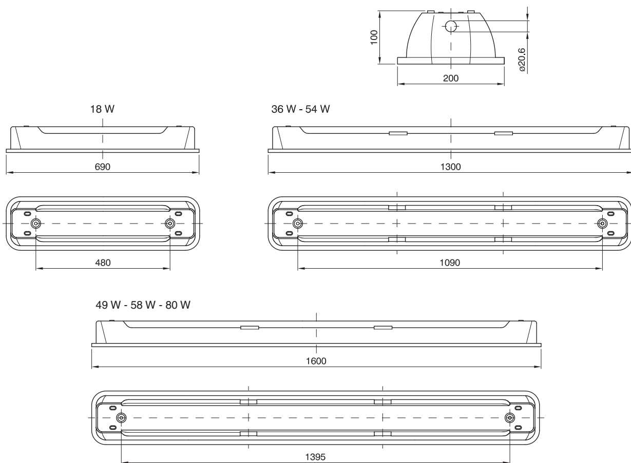
RINO series - Watertight lighting fixtures with glass diffuser
