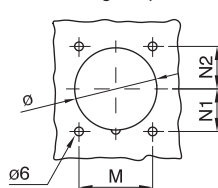
Drilling template
