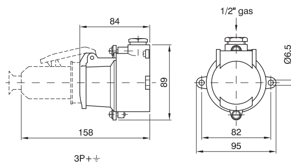
RONDÒ series - Protected wall-mounted industrial socket-outlets
