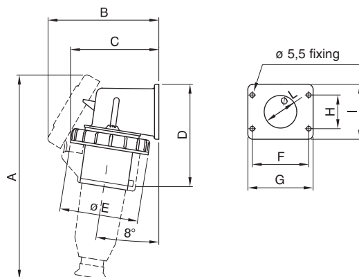
CEE series - Protected 90° angled plugs
