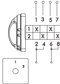
CAM 41 - Voltmetric three concatenated voltages-two of phase
