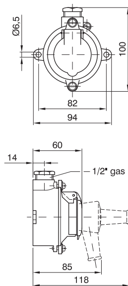
RONDÒ series - Protected wall-mounted industrial socket-outlets
