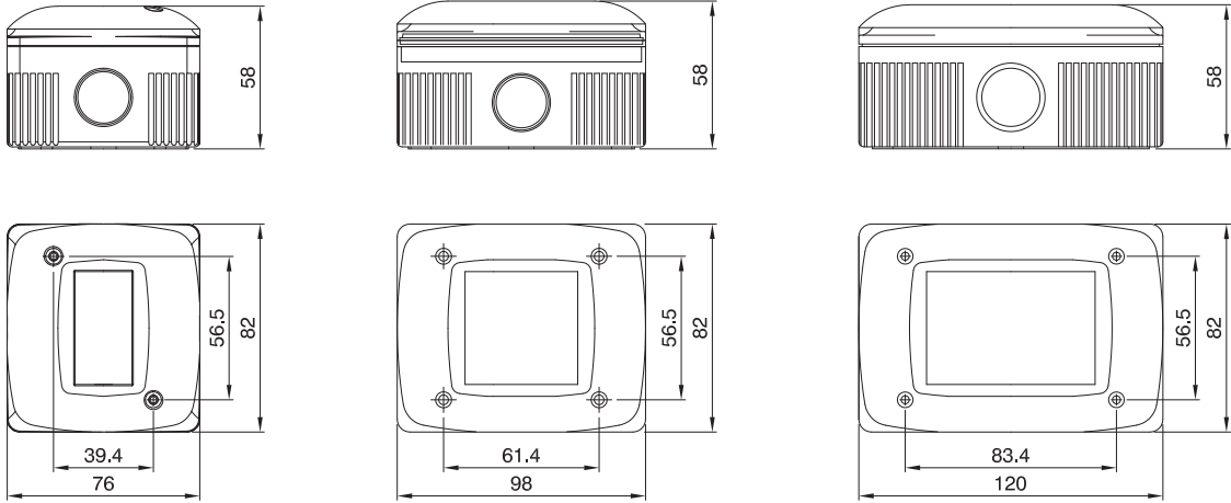
DomoTER series protected wall-mounted enclosures
