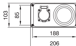
Socket-outlet with transformer cod. 494024 cod. 496024
