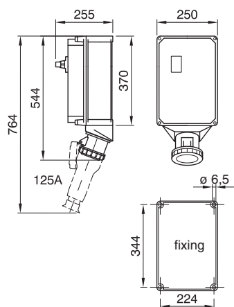
TAIS series - Wall-mounted socket-outlets with automatic circuit breaker, electrical and differential interlock
