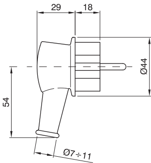
SPIN series - German standard protected plug in impact-proof rubber IP44
