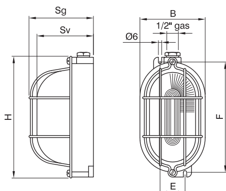
RINO series - Watertight pendant and ceiling installation lighting fixtures
