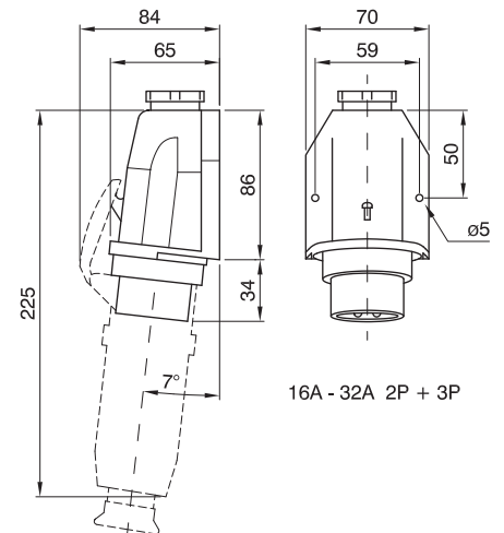
CEE series - Protected 90° angled plugs very low voltage
