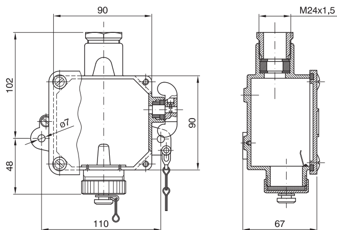
NAVE series - Socket-outlets UNAV 1436
