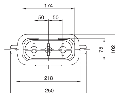
FP series - Watertight plug with aligned poles
