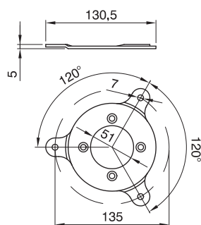
NAUTILUX series - Pendant lamp IP22
