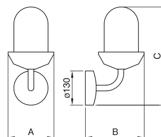
NAUTILUX series - Brass wall lighting fixtures IP44
