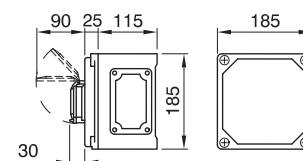
TAIS / TAIS-Ex series Boxes for combinations
