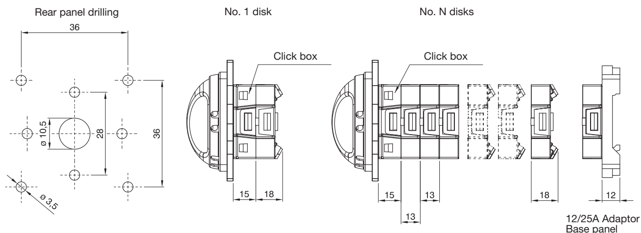
CAM-ST series - Rear panel rotary control devices 12/25A
