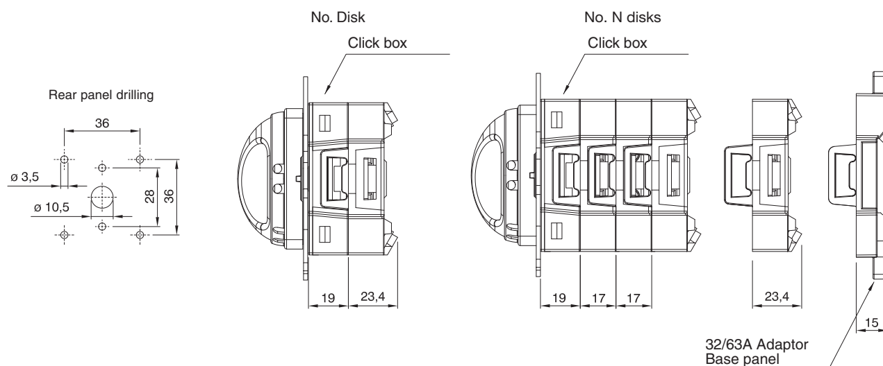
CAM-ST series - Rear and base panel rotary control devices 32/63A
