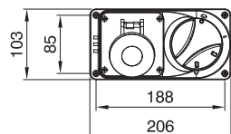
16A/32A - IP44/IP55
