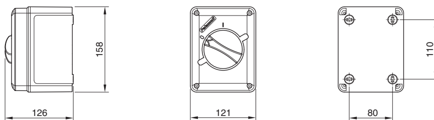
CAM-ST series - 16A and 32A isolator switches in thermoplastic enclosure
