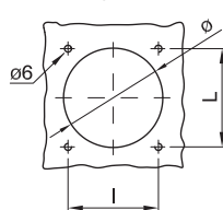
Drilling template
