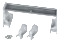
topTER SERIES DIN EN50022 Guide kit for topTER distribution boards
