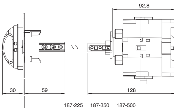
CAM-SZ series - Isolators 40A÷100A with base panel doorlock
