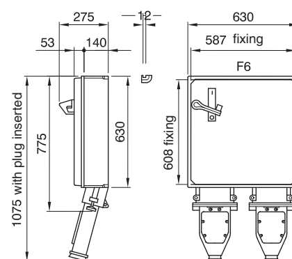
FP ALUPRES series -Wall-mounted interlocked socket-outlets
