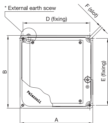
TUNNEL series - 63A plugs and socket-outlets for tunnel jettfans
