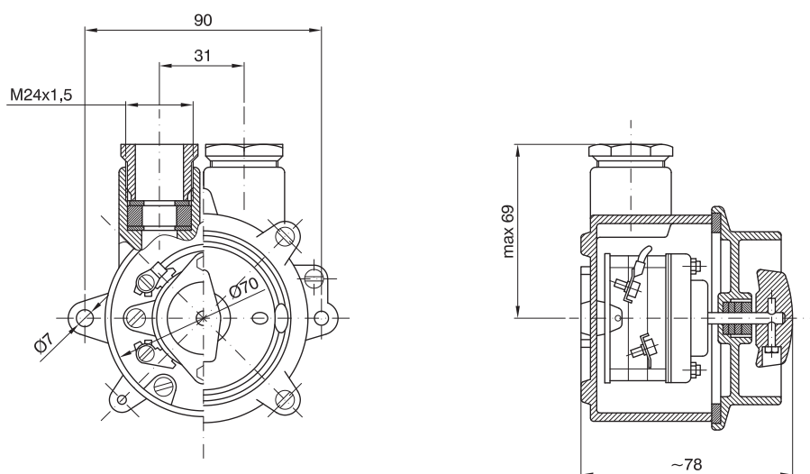
NAVE series - Watertight brass switches and two-way switches UNAV 2162
