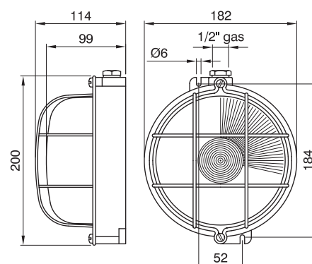
RINO/RINO-Ex series Watertight round luminaires
