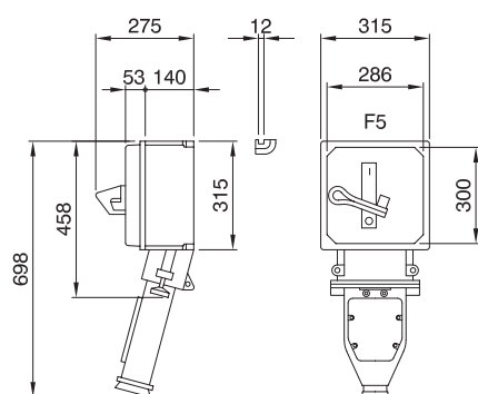
TUNNEL series - 63A plugs and socket-outlets for tunnel jettfans
