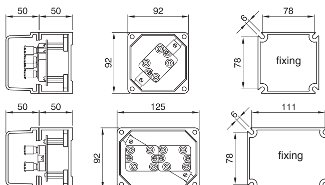
NAVE series - Junction boxes UNAV 2181
