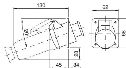
Drilling template
