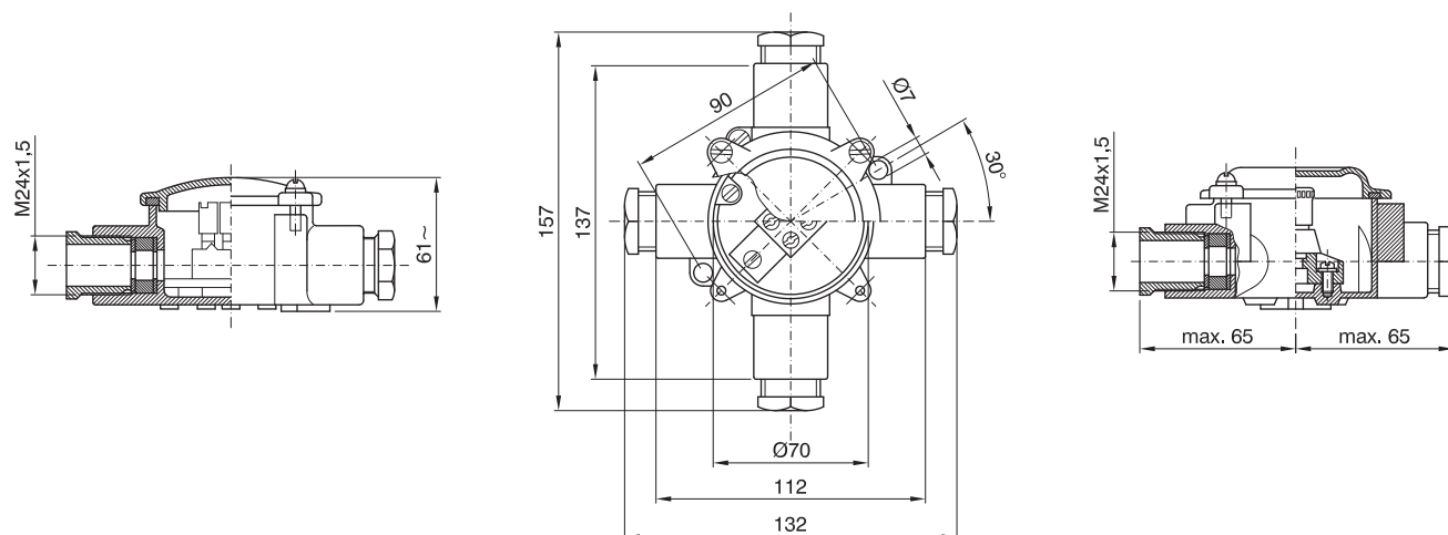
NAVE series - Junction boxes UNAV 1401, UNAV 1398
