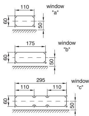
TAIS series - Modular box windows
