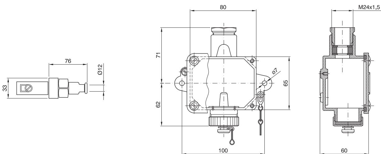
NAVE series - Plugs UNAV 1437
