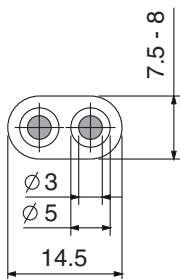
Cable section 6 mm 2 for 32A plugs
