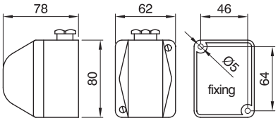
TAIS-MIGNON / TAIS-MIGNON-Ex series Signal lamps in wall-mounting watertight enclosure
