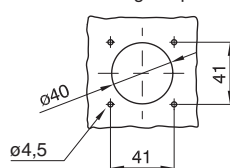
Drilling template
