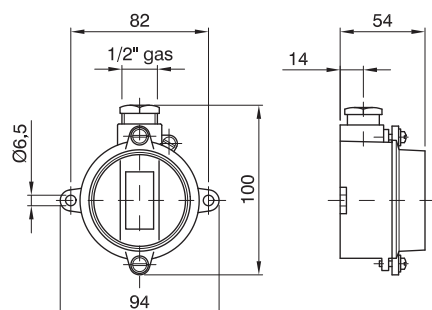
RONDÒ / RONDÒ-Ex series - Switches, two-way switches and selector switches in wall-mounted watertight enclosure
