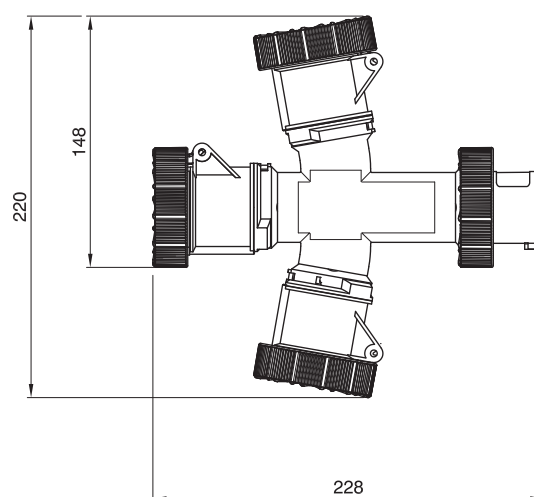
3 gang watertight multipliers
