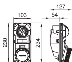
3P+N+16A
